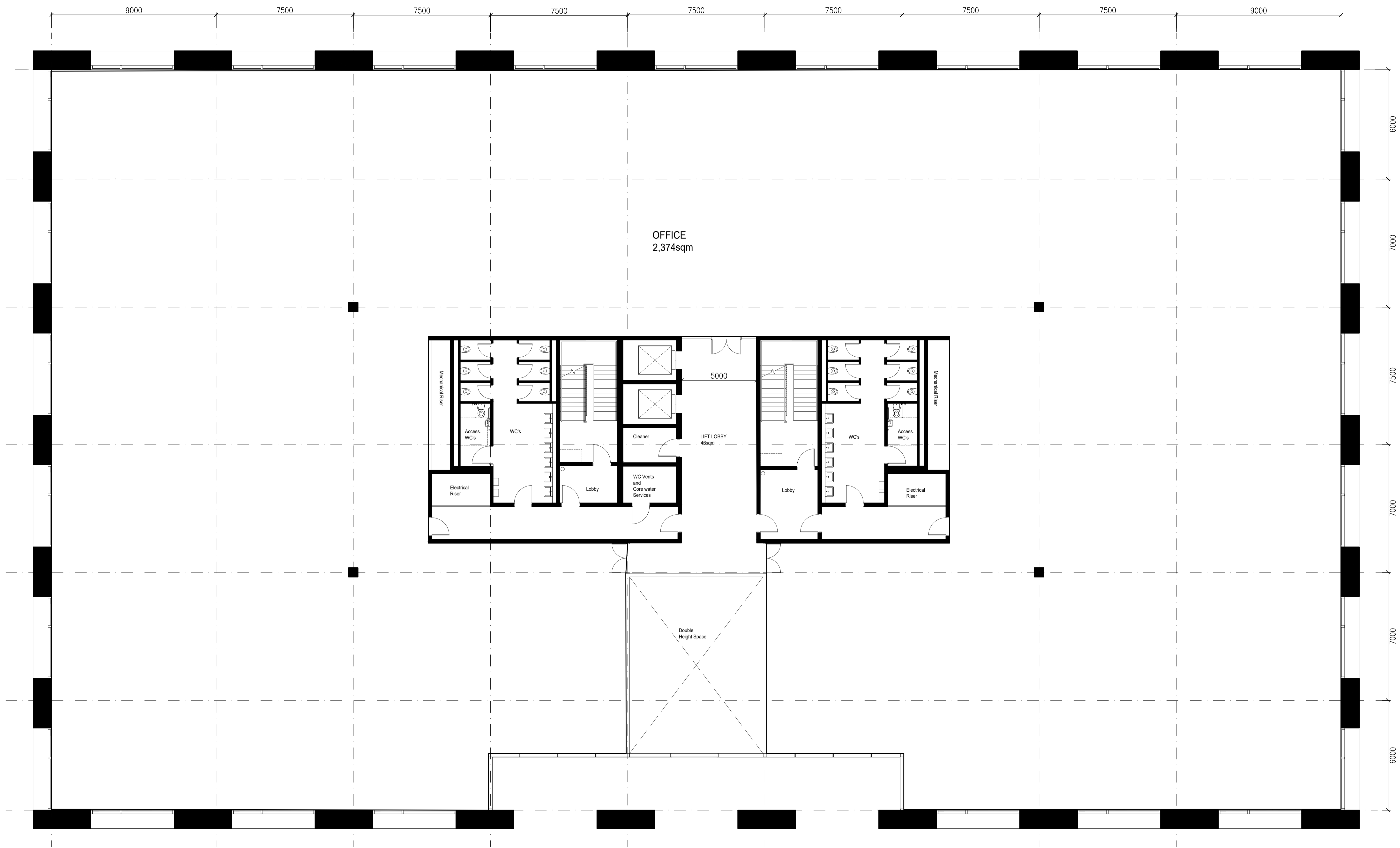
01 | First Floor Plan 1:100
