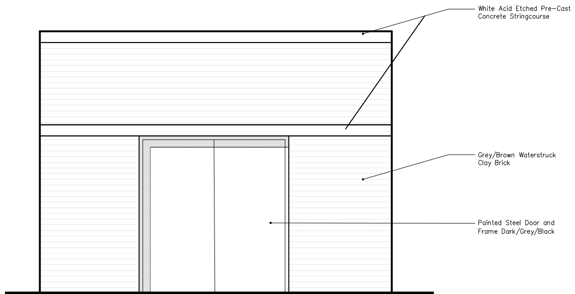
03 West Elevation 1:50
